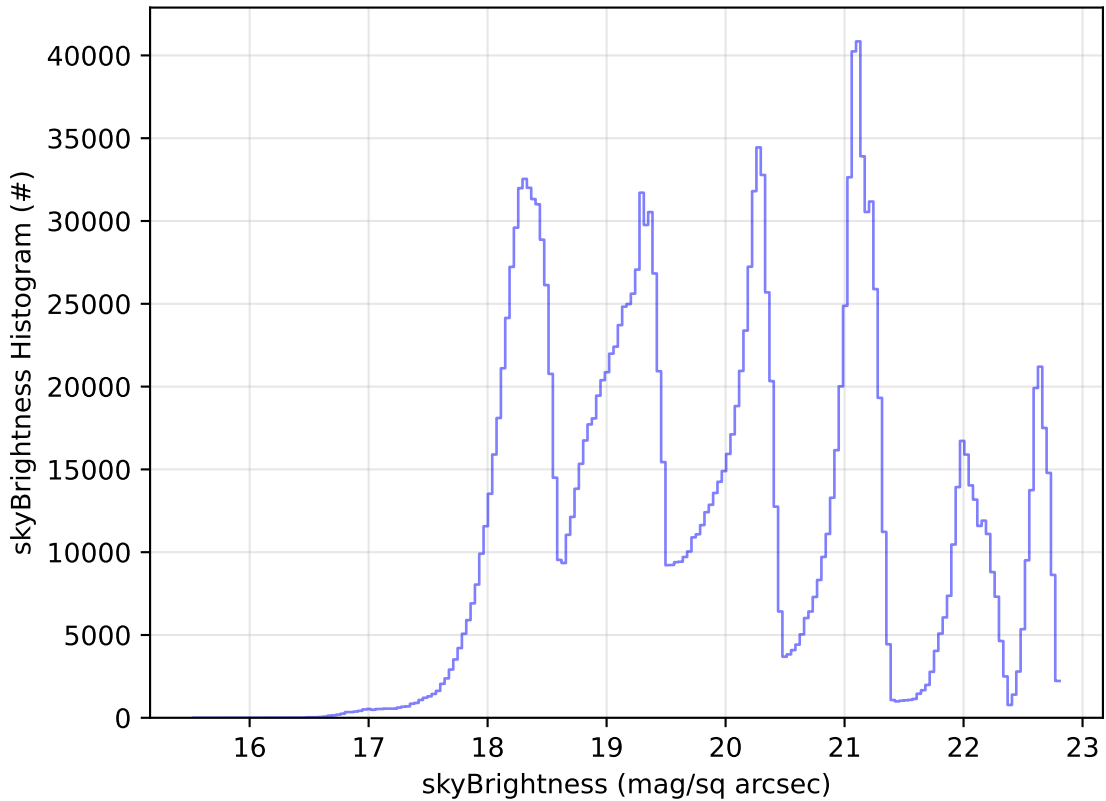
ddf_acor_sf10_lsf20_lsr50_v3.4_10yrs All sky all bands: skyBrightness Histogram
