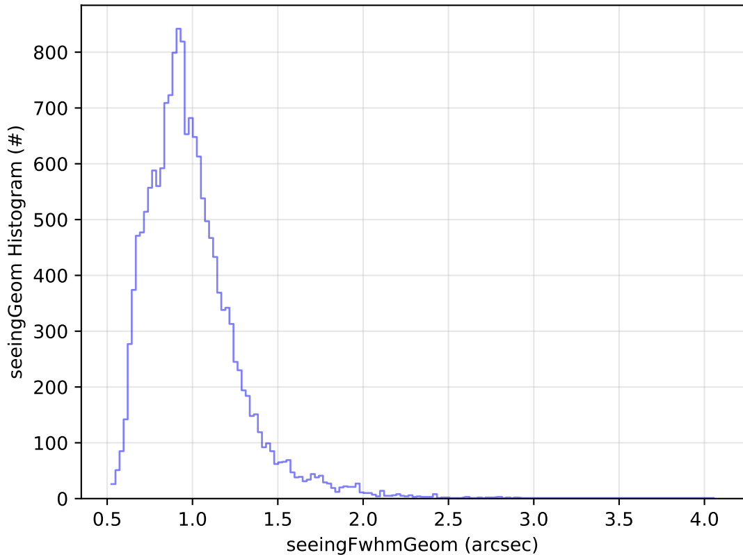
ddf_acor_sf10_lsf20_lsr50_v3.4_10yrs Yr 1 u band: seeingGeom Histogram
