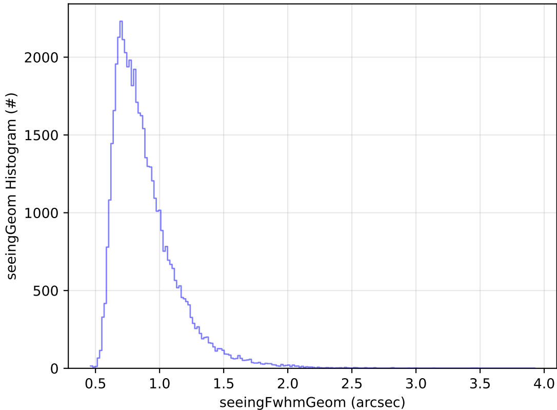
ddf_acor_sf10_lsf20_lsr50_v3.4_10yrs Yr 1 r band: seeingGeom Histogram
