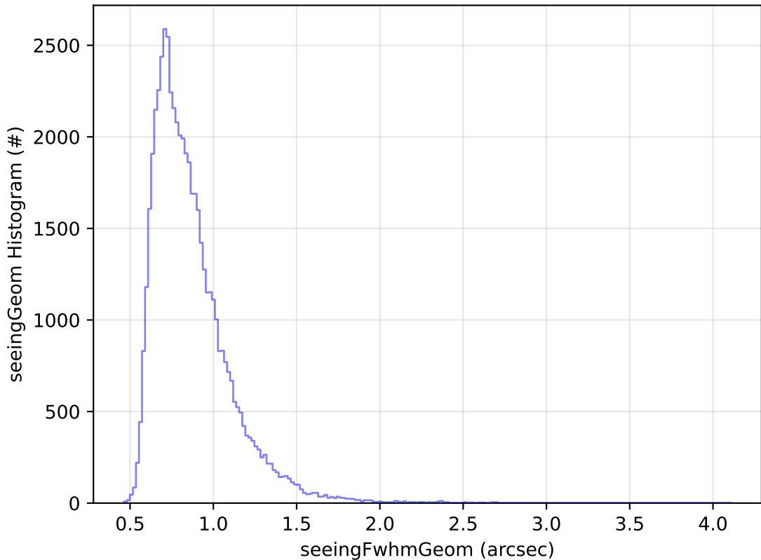
ddf_acor_sf10_lsf20_lsr50_v3.4_10yrs Yr 1 i band: seeingGeom Histogram
