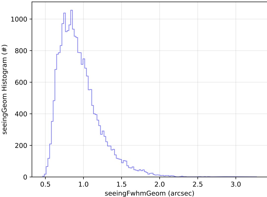
ddf_acor_sf10_lsf20_lsr50_v3.4_10yrs Yr 1 g band: seeingGeom Histogram
