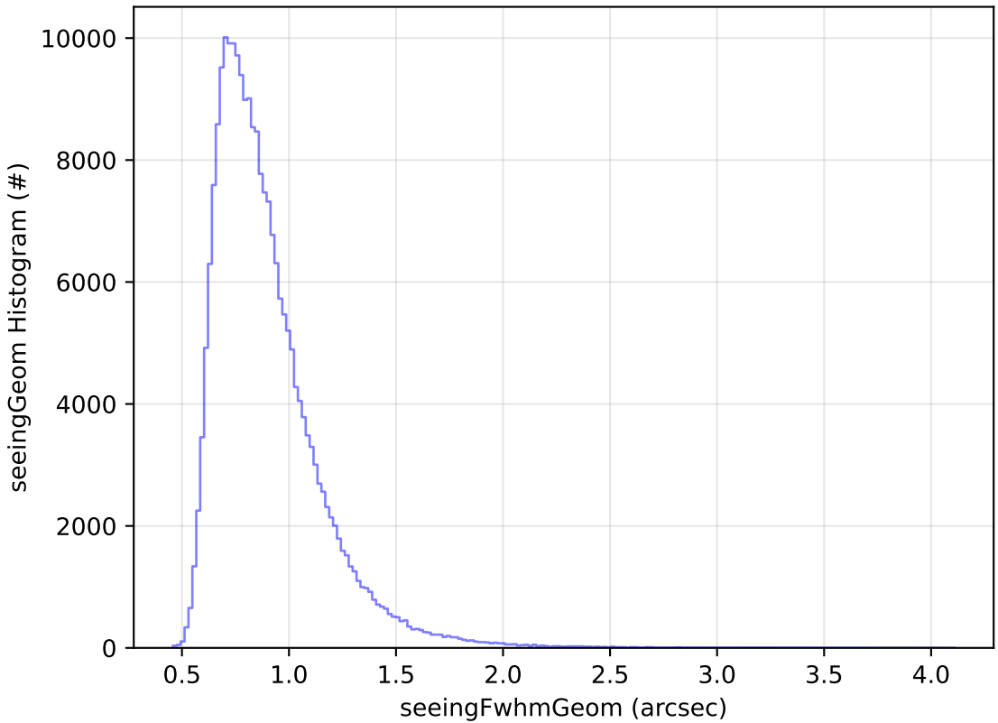
ddf_acor_sf10_lsf20_lsr50_v3.4_10yrs Yr 1 all bands: seeingGeom Histogram
