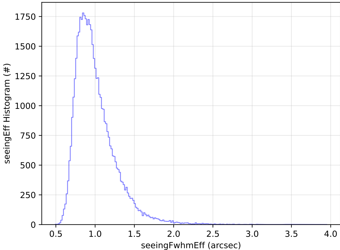
ddf_acor_sf10_lsf20_lsr50_v3.4_10yrs Yr 1 y band: seeingEff Histogram
