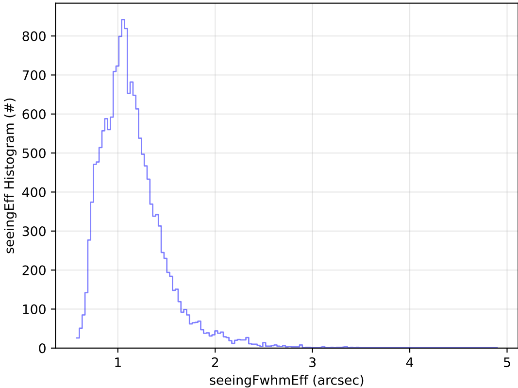
ddf_acor_sf10_lsf20_lsr50_v3.4_10yrs Yr 1 u band: seeingEff Histogram
