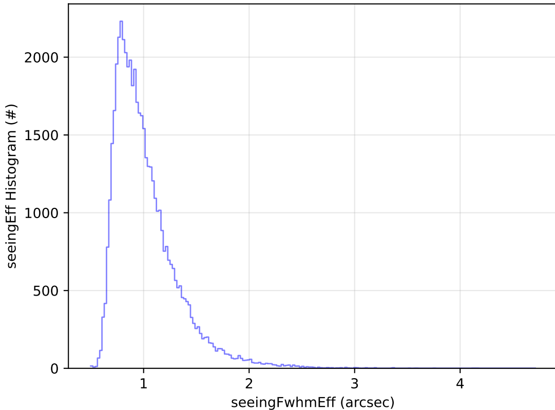
ddf_acor_sf10_lsf20_lsr50_v3.4_10yrs Yr 1 r band: seeingEff Histogram
