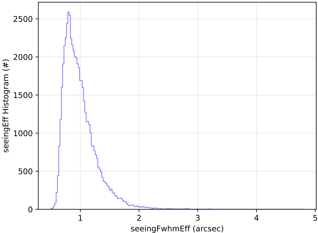
ddf_acor_sf10_lsf20_lsr50_v3.4_10yrs Yr 1 i band: seeingEff Histogram
