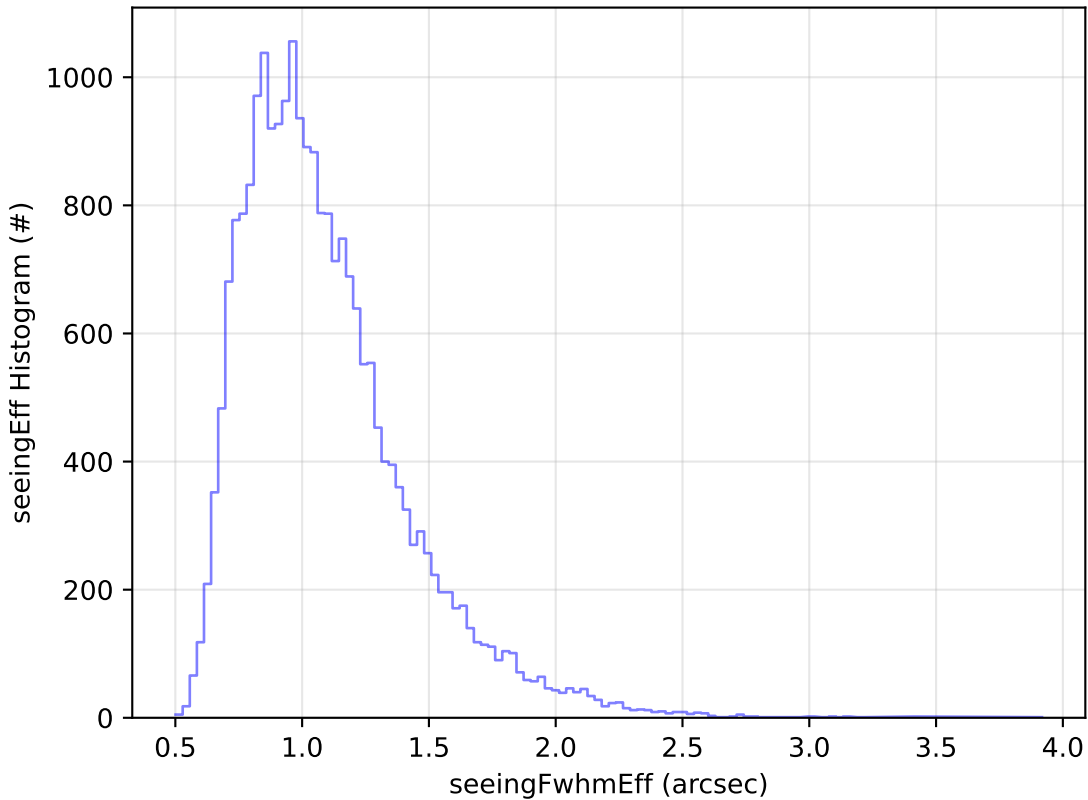
ddf_acor_sf10_lsf20_lsr50_v3.4_10yrs Yr 1 g band: seeingEff Histogram
