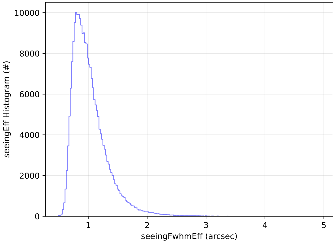
ddf_acor_sf10_Isf20_Isr50_v3.4_10yrs Yr 1 all bands: seeingEff Histogram
