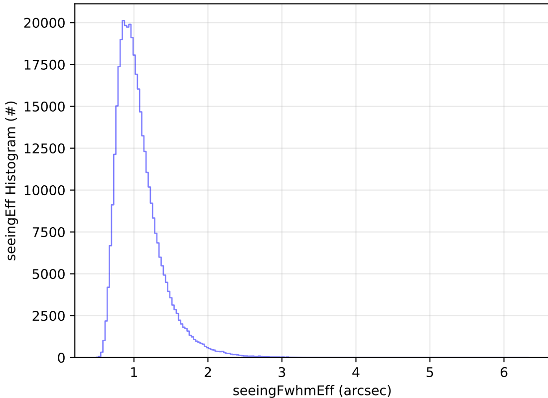
ddf_acor_sf10_lsf20_lsr50_v3.4_10yrs WFD y band: seeingEff Histogram
