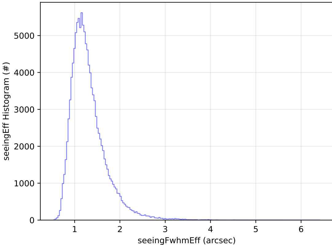
ddf_acor_sf10_lsf20_lsr50_v3.4_10yrs WFD u band: seeingEff Histogram
