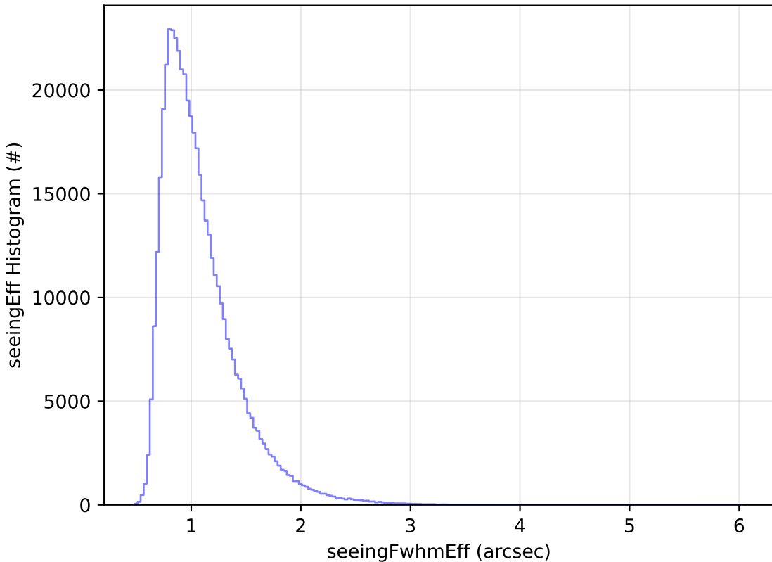
ddf_acor_sf10_lsf20_lsr50_v3.4_10yrs WFD i band: seeingEff Histogram
