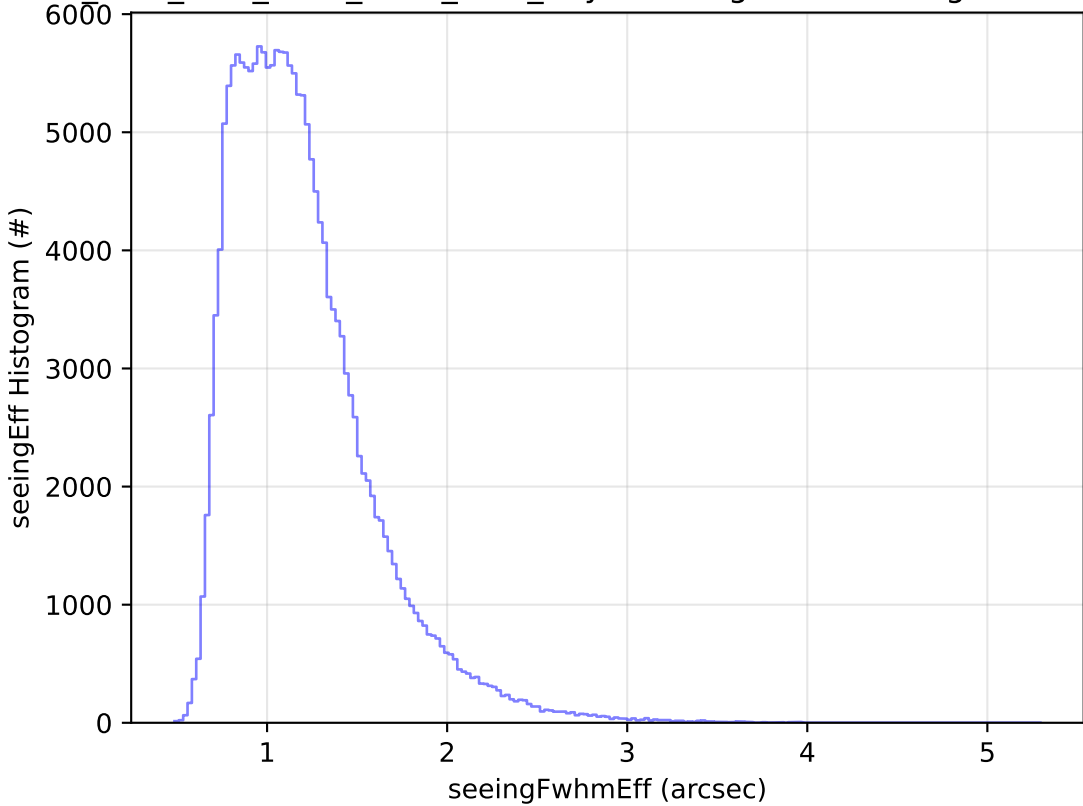
ddf_acor_sf10_lsf20_lsr50_v3.4_10yrs WFD g band: seeingEff Histogram
