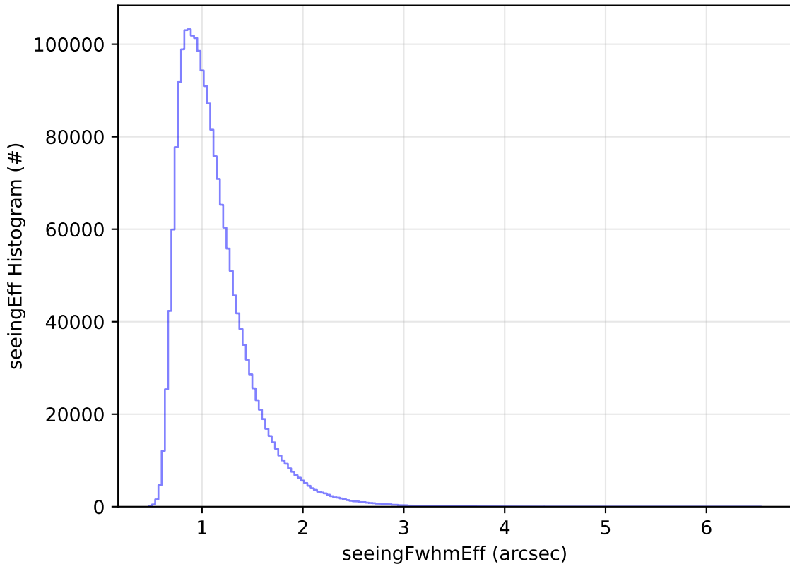
ddf_acor_sf10_lsf20_lsr50_v3.4_10yrs WFD all bands: seeingEff Histogram
