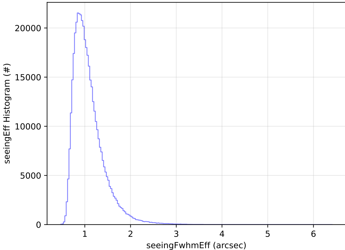
ddf_acor_sf10_lsf20_lsr50_v3.4_10yrs All sky z band: seeingEff Histogram
