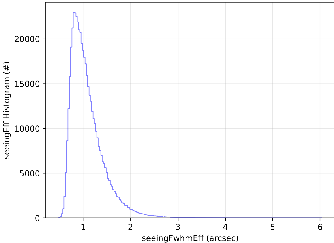
ddf_acor_sf10_lsf20_lsr50_v3.4_10yrs All sky i band: seeingEff Histogram
