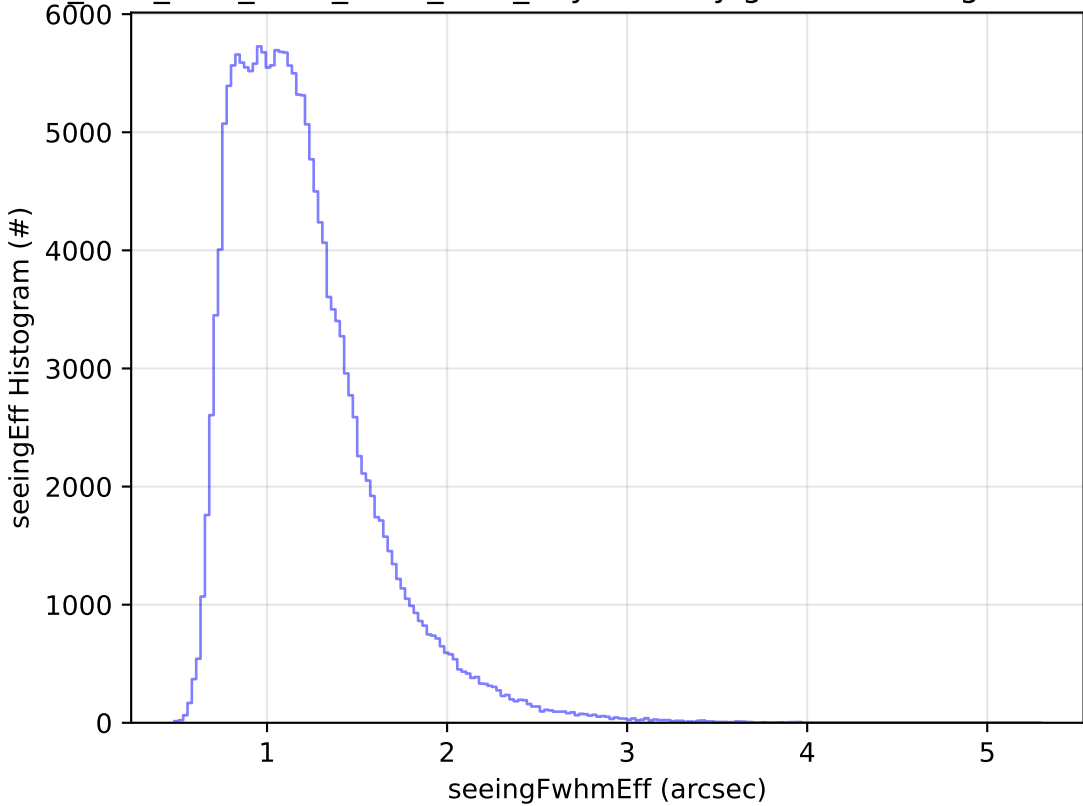
ddf_acor_sf10_ls20_lsr50_v3.4_10yrs All sky g band: seeingEff Histogram
