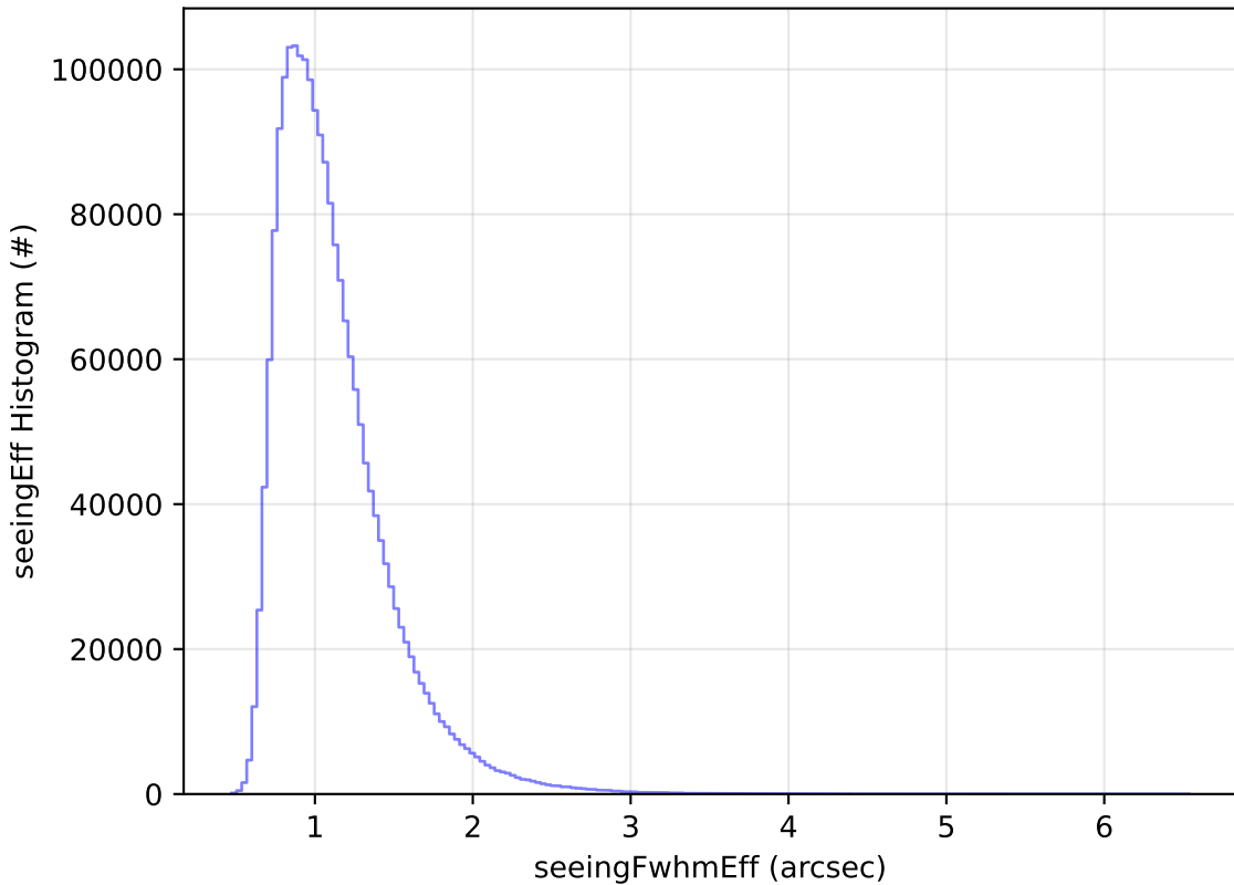
ddf_acor_sf10_lsf20_lsr50_v3.4_10yrs All sky all bands: seeingEff Histogram
