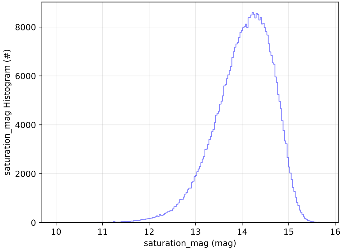
ddf_acor_sf10_lsf20_lsr50_v3.4_10yrs WFD z band: saturation_mag Histogram
