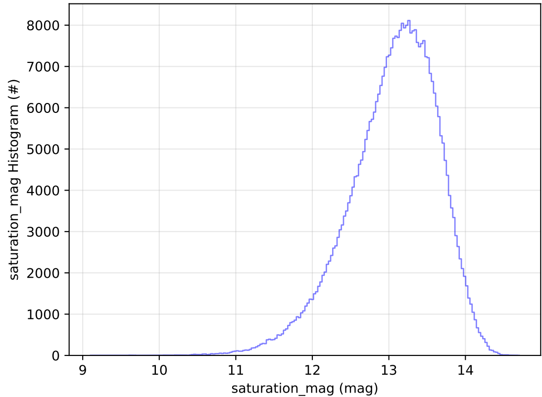
ddf_acor_sf10_lsf20_lsr50_v3.4_10yrs WFD y band: saturation_mag Histogram
