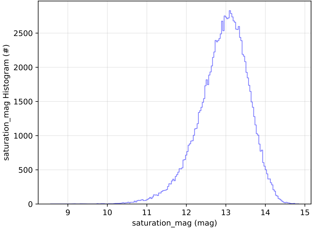
ddf_acor_sf10_lsf20_lsr50_v3.4_10yrs WFD u band: saturation_mag Histogram
