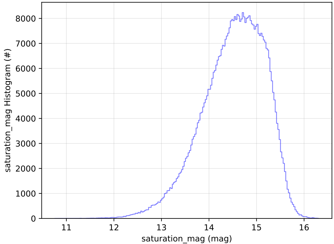
ddf_acor_sf10_lsf20_lsr50_v3.4_10yrs WFD r band: saturation_mag Histogram
