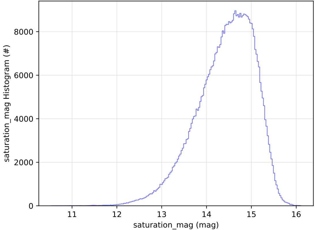
ddf_acor_sf10_lsf20_lsr50_v3.4_10yrs WFD i band: saturation_mag Histogram
