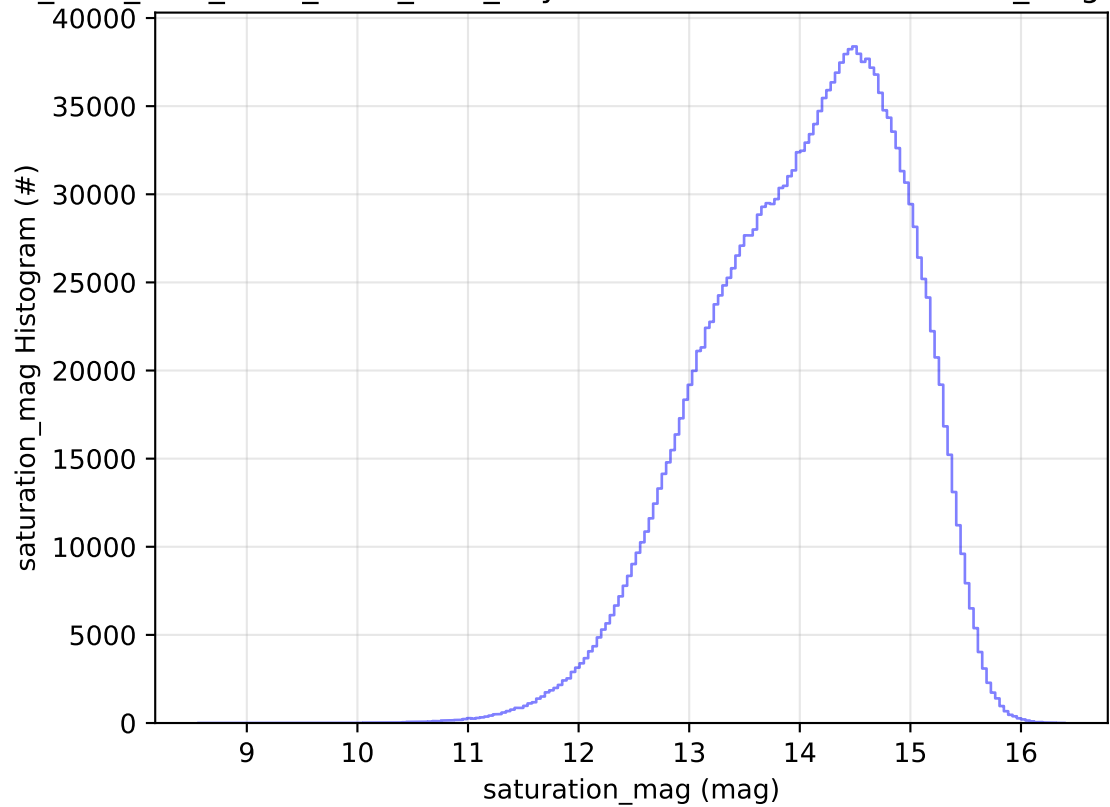
ddf_acor_sf10_lsf20_lsr50_v3.4_10yrs WFD all bands: saturation_mag Histogram
