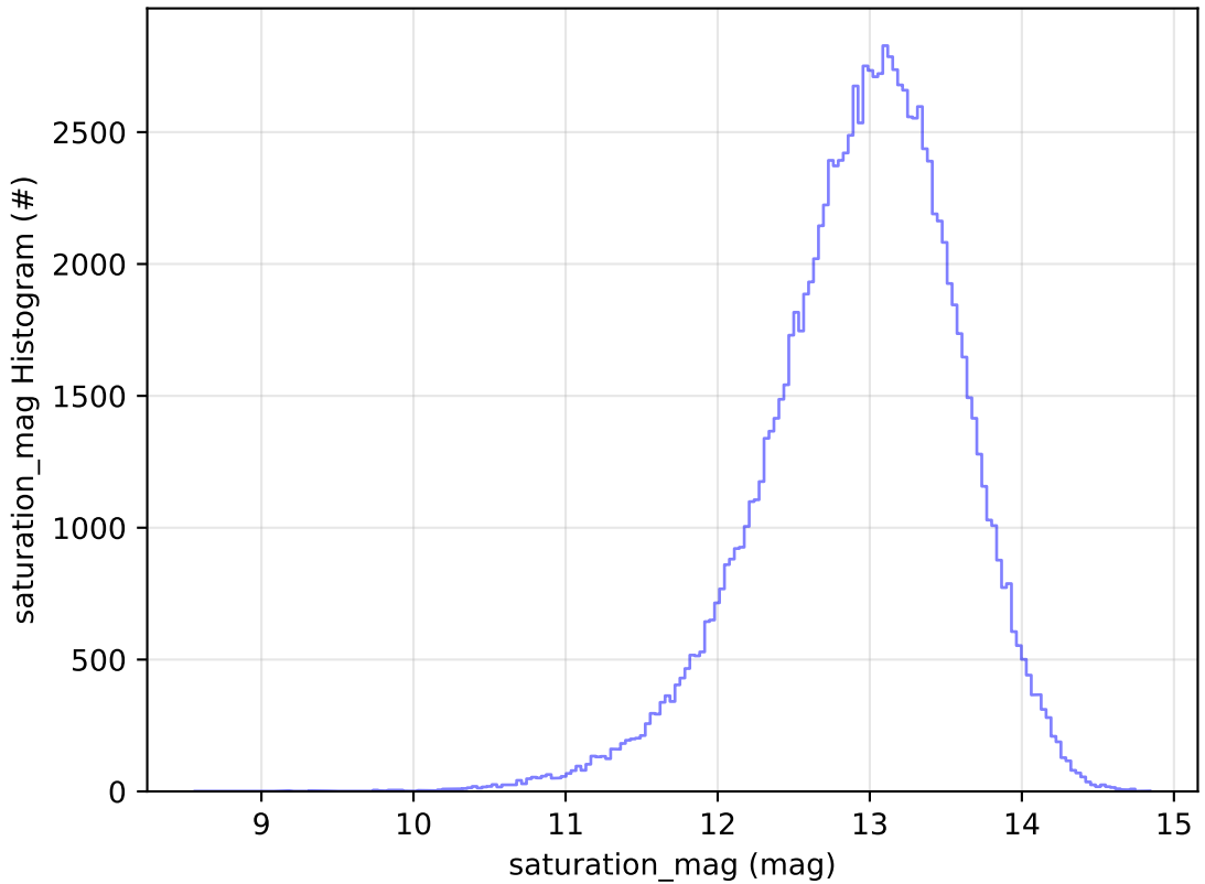
ddf_acor_sf10_lsf20_lsr50_v3.4_10yrs All sky u band: saturation_mag Histogram
