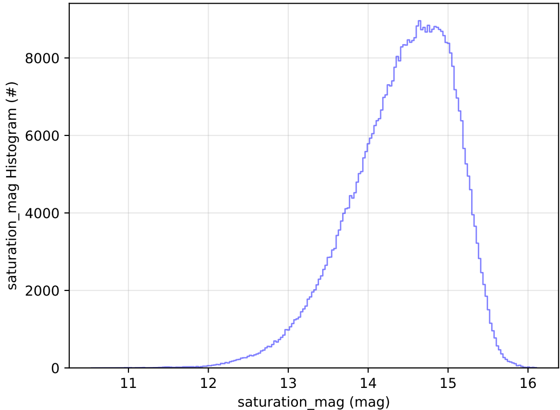
ddf_acor_sf10_lsf20_lsr50_v3.4_10yrs All sky i band: saturation_mag Histogram
