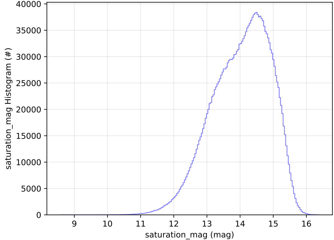
ddf_acor_sf10_lsf20_lsr50_v3.4_10yrs All sky all bands: saturation_mag Histogram
