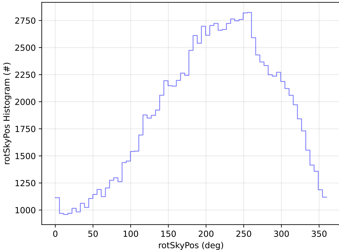
ddf_acor_sf10_lsf20_lsr50_v3.4_10yrs WFD u band: rotSkyPos Histogram
