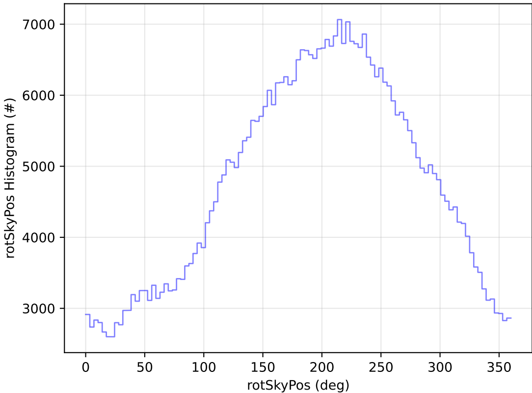
ddf_acor_sf10_lsf20_lsr50_v3.4_10yrs WFD r band: rotSkyPos Histogram
