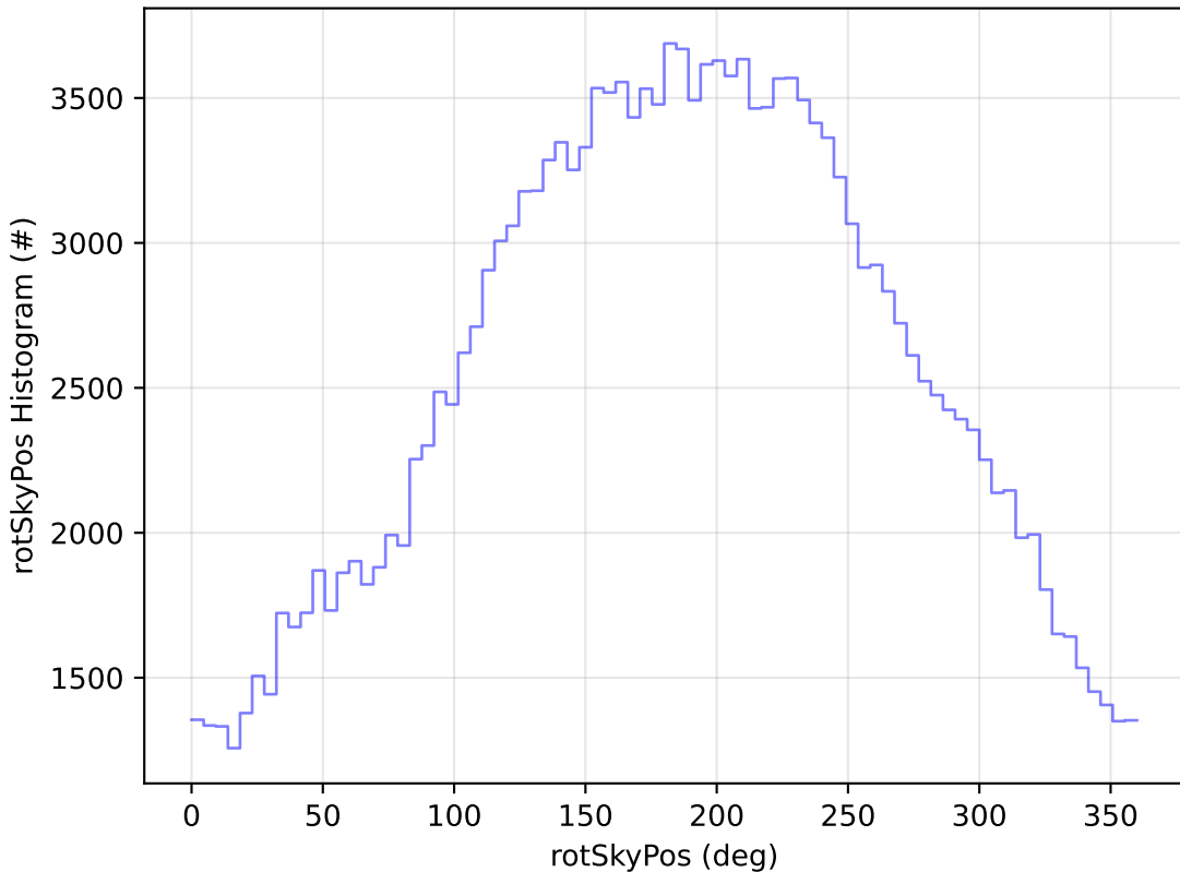
ddf_acor_sf10_lsf20_lsr50_v3.4_10yrs WFD g band: rotSkyPos Histogram
