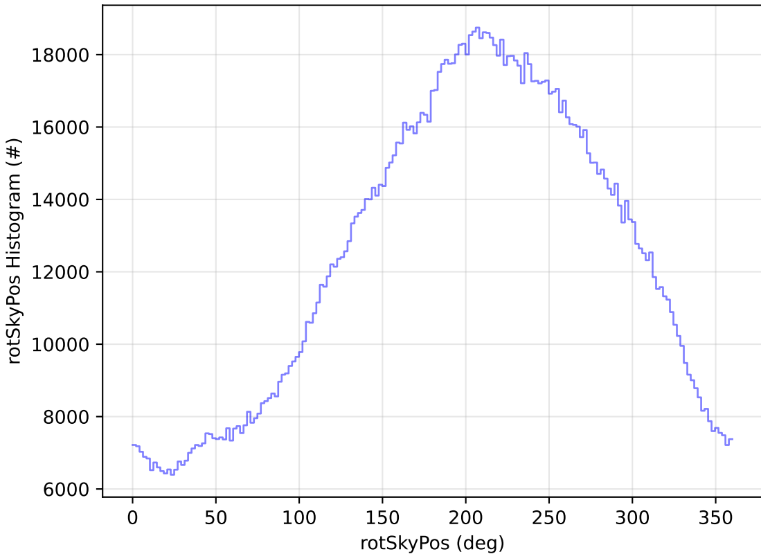
ddf_acor_sf10_lsf20_lsr50_v3.4_10yrs WFD all bands: rotSkyPos Histogram
