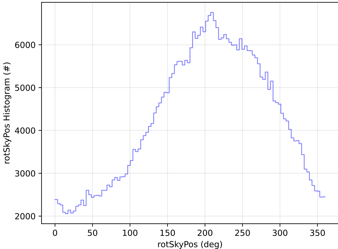
ddf_acor_sf10_lsf20_lsr50_v3.4_10yrs All sky z band: rotSkyPos Histogram
