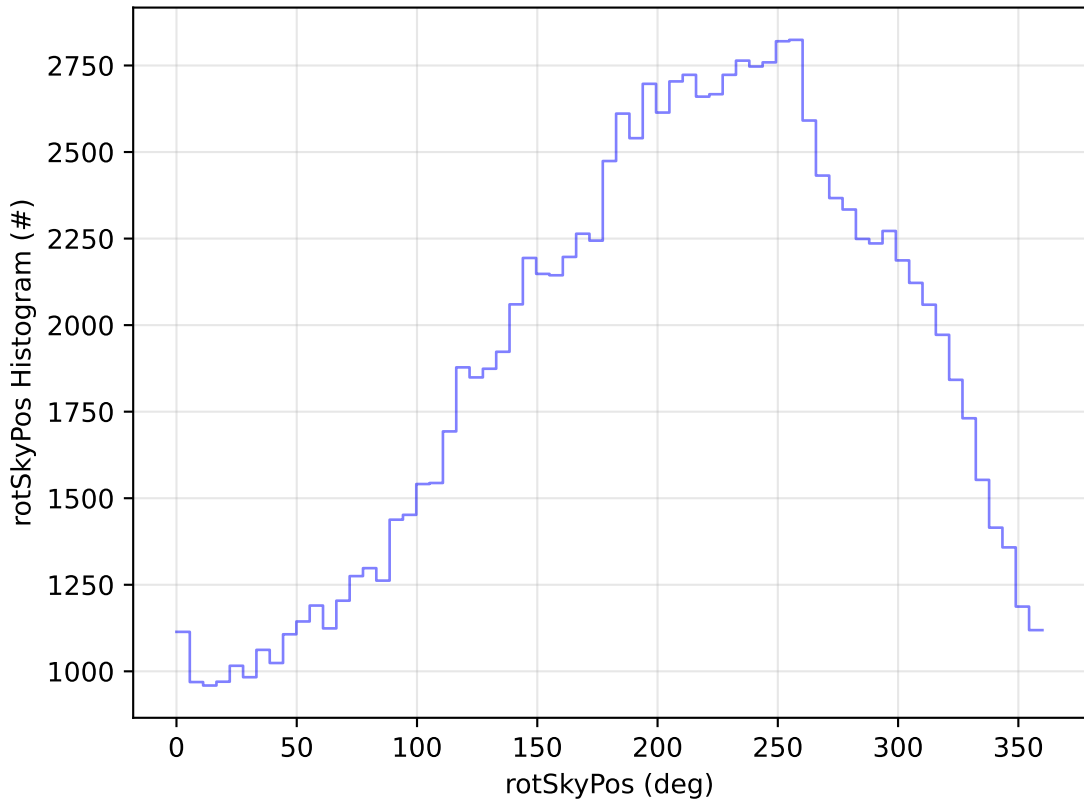
ddf_acor_sf10_lsf20_lsr50_v3.4_10yrs All sky u band: rotSkyPos Histogram
