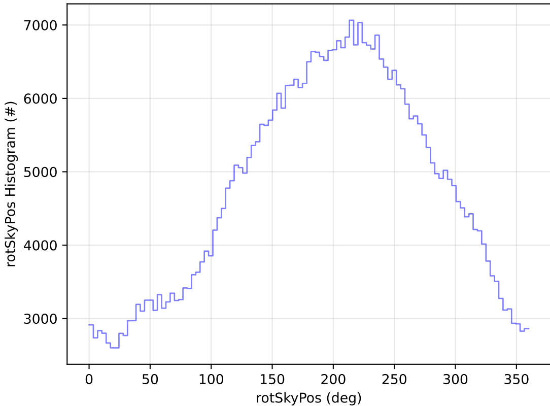
ddf_acor_sf10_lsf20_lsr50_v3.4_10yrs All sky r band: rotSkyPos Histogram
