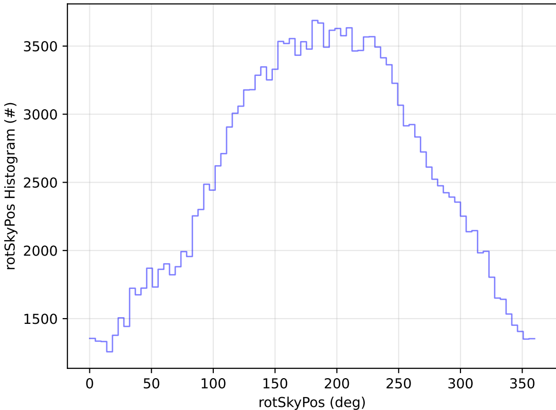
ddf_acor_sf10_lsf20_lsr50_v3.4_10yrs All sky g band: rotSkyPos Histogram
