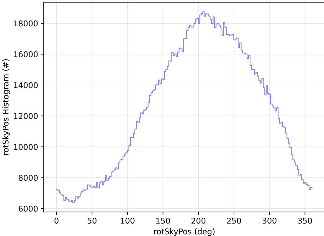
ddf_acor_sf10_lsf20_lsr50_v3.4_10yrs All sky all bands: rotSkyPos Histogram
