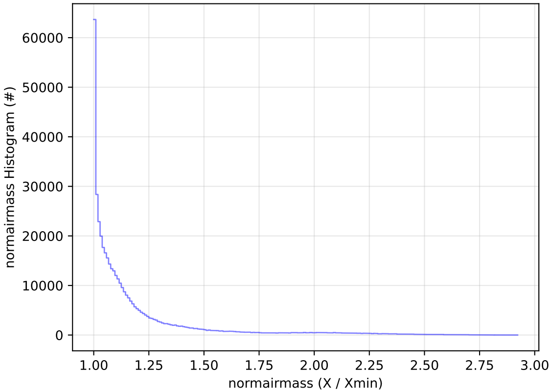
ddf_acor_sf10_lsf20_lsr50_v3.4_10yrs WFD z band: normairmass Histogram
