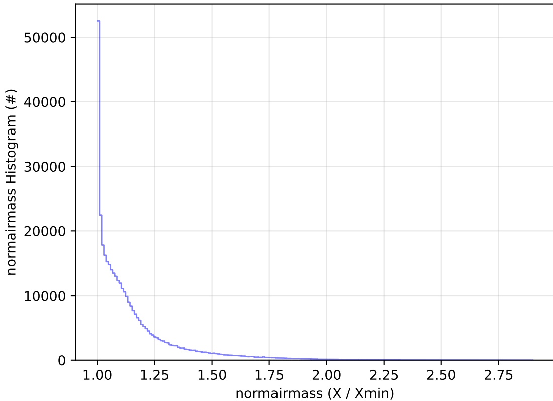
ddf_acor_sf10_lsf20_lsr50_v3.4_10yrs WFD y band: normairmass Histogram
