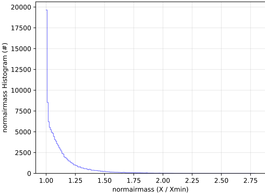
ddf_acor_sf10_lsf20_lsr50_v3.4_10yrs WFD u band: normairmass Histogram
