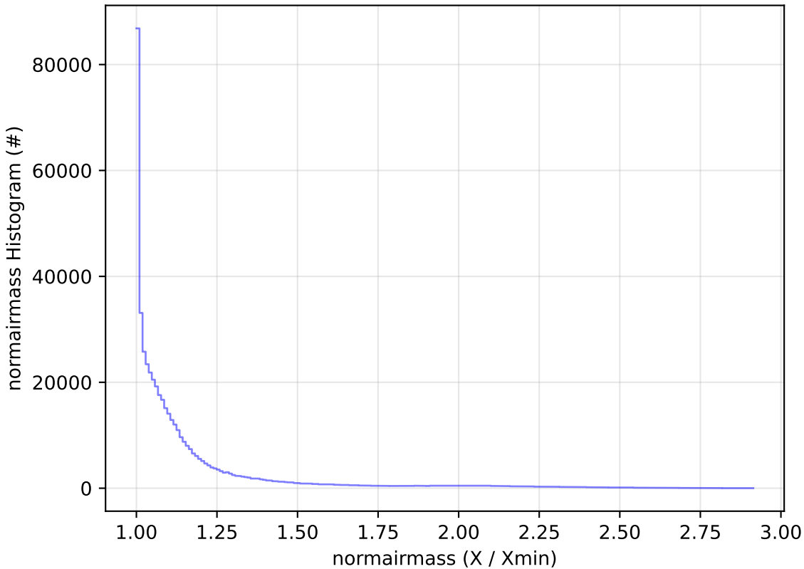
ddf_acor_sf10_lsf20_lsr50_v3.4_10yrs WFD i band: normairmass Histogram
