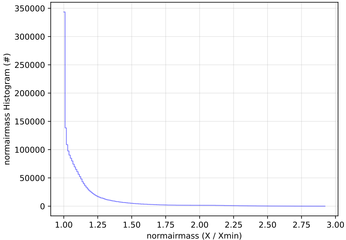
ddf_acor_sf10_lsf20_lsr50_v3.4_10yrs WFD all bands: normairmass Histogram
