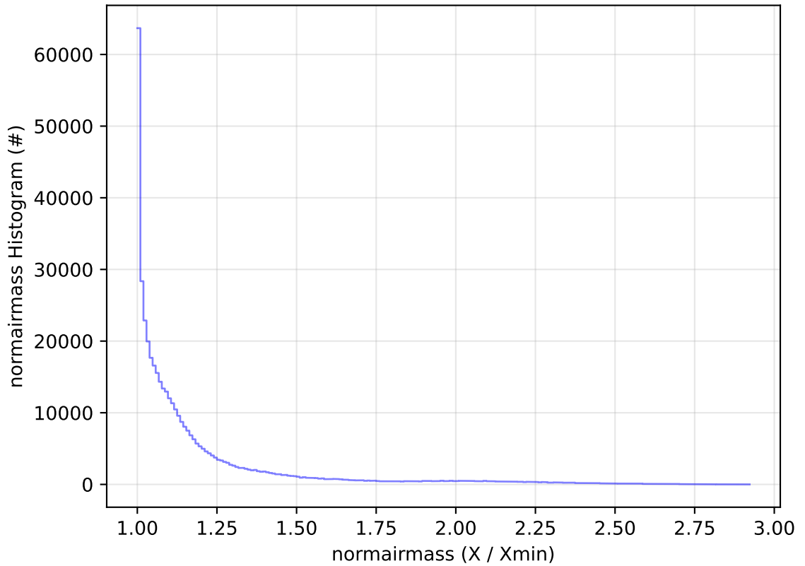
ddf_acor_sf10_lsf20_lsr50_v3.4_10yrs All sky z band: normairmass Histogram
