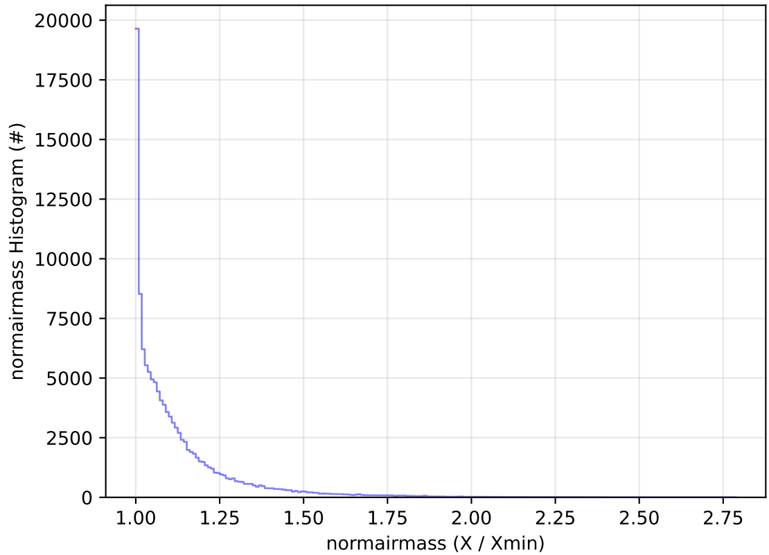
ddf_acor_sf10_lsf20_lsr50_v3.4_10yrs All sky u band: normairmass Histogram
