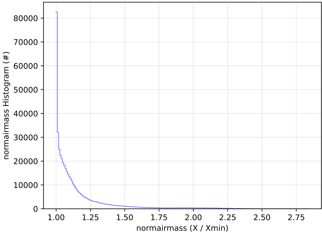
ddf_acor_sf10_lsf20_lsr50_v3.4_10yrs All sky r band: normairmass Histogram
