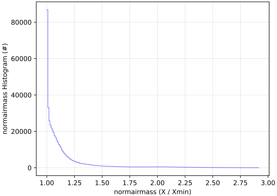
ddf_acor_sf10_lsf20_lsr50_v3.4_10yrs All sky i band: normairmass Histogram
