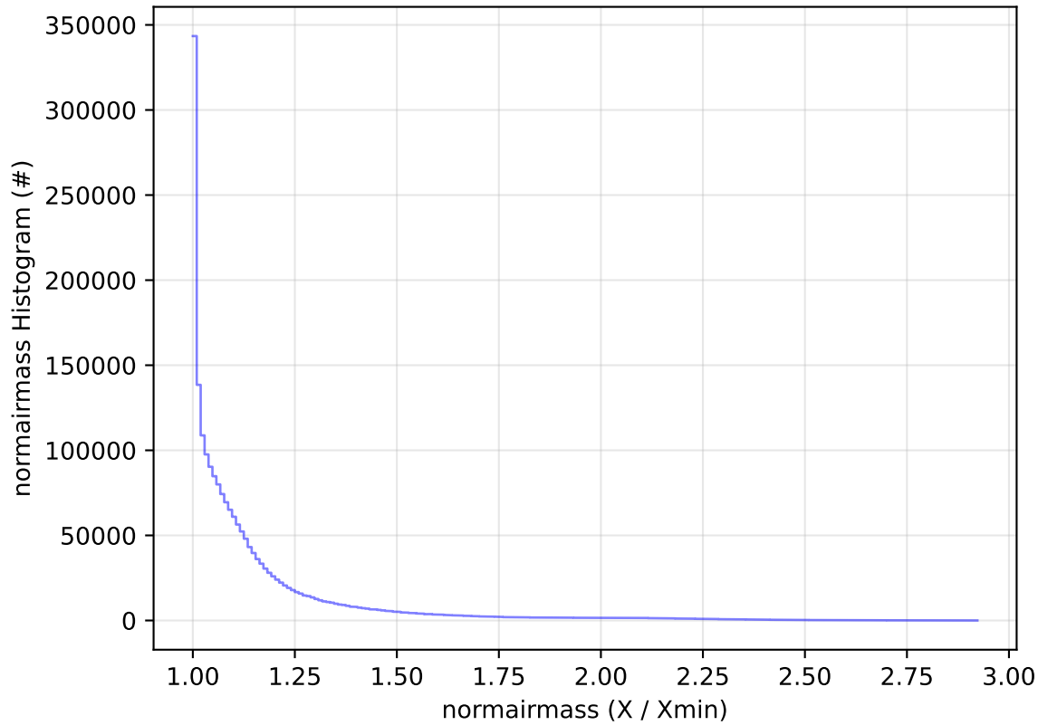
ddf_acor_sf10_lsf20_lsr50_v3.4_10yrs All sky all bands: normairmass Histogram
