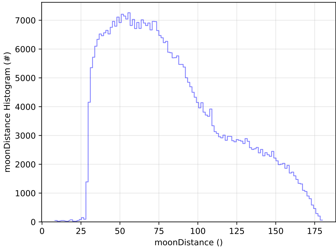
ddf_acor_sf10_lsf20_lsr50_v3.4_10yrs WFD z band: moonDistance Histogram
